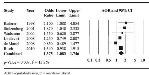
Figure 2. Forest plot of pooled adjusted odds ratio.
