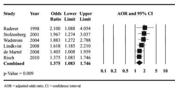
Figure 4. Cumulative meta-analysis results.
